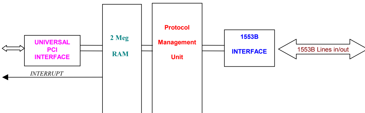
Figure 1-1. IIB-1553-PC104+ Functional Block Diagram
