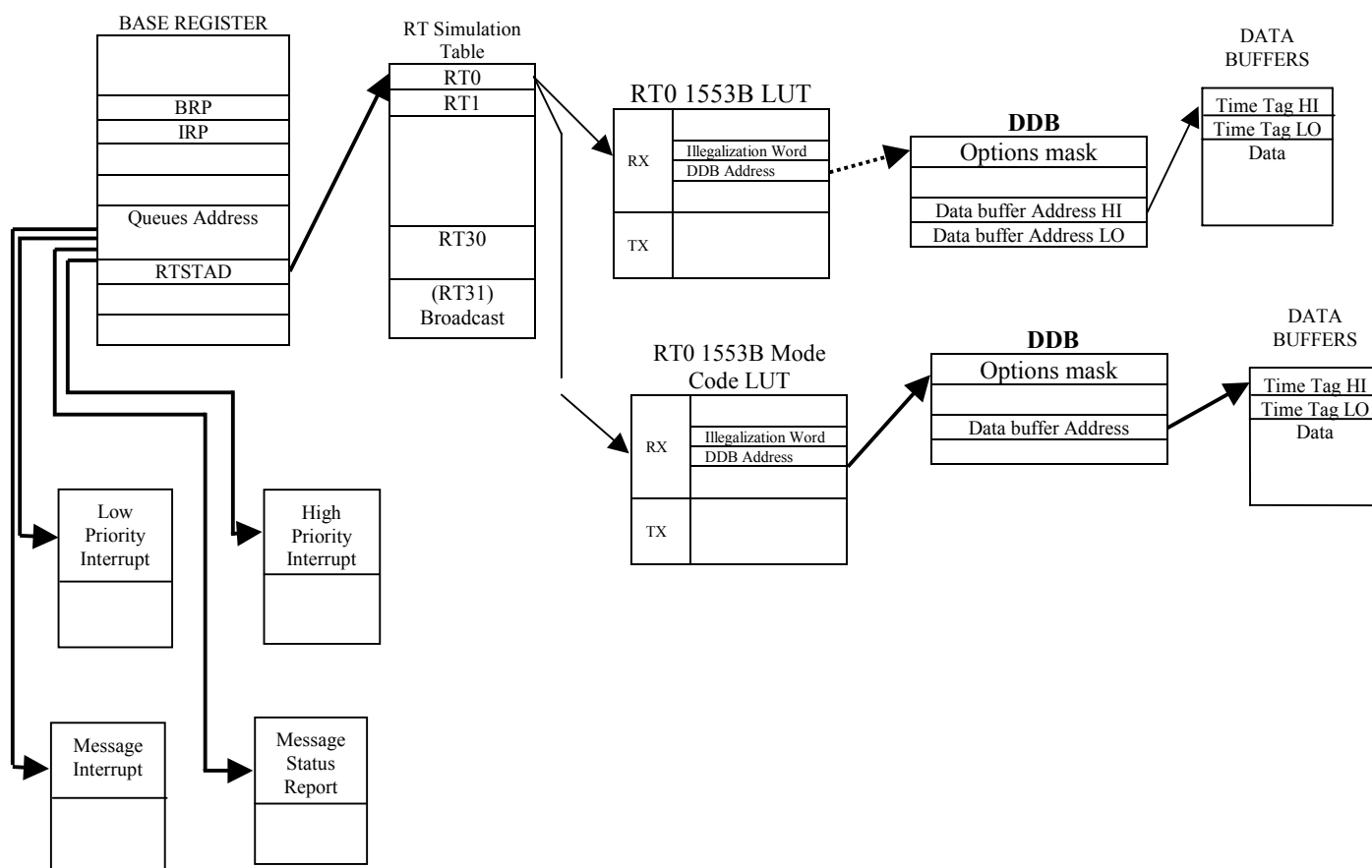
Figure 5-1 Multiple Remote Terminal Organisation Diagram
