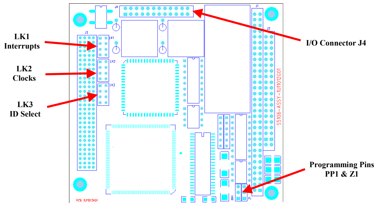
Figure 1-2. IIB-1553-PC104+ Layout Diagram
