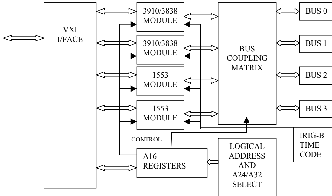
Figure 1-1 VXI-2800 Motherboard Functional Block Diagram
