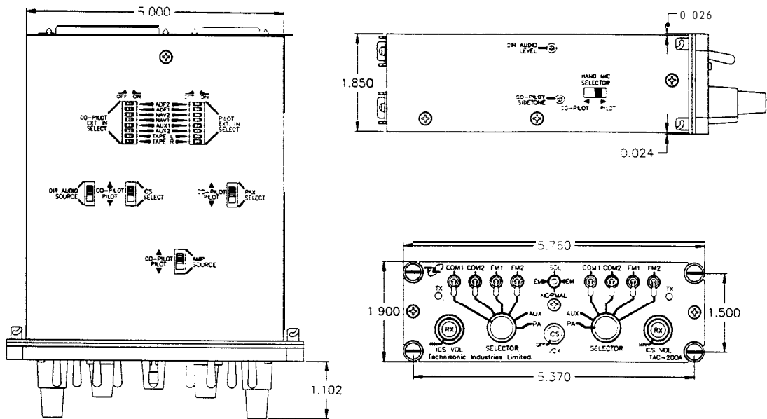
FIGURE 2-1 Outline Drawing for Model TAC-200A Audio Controller
