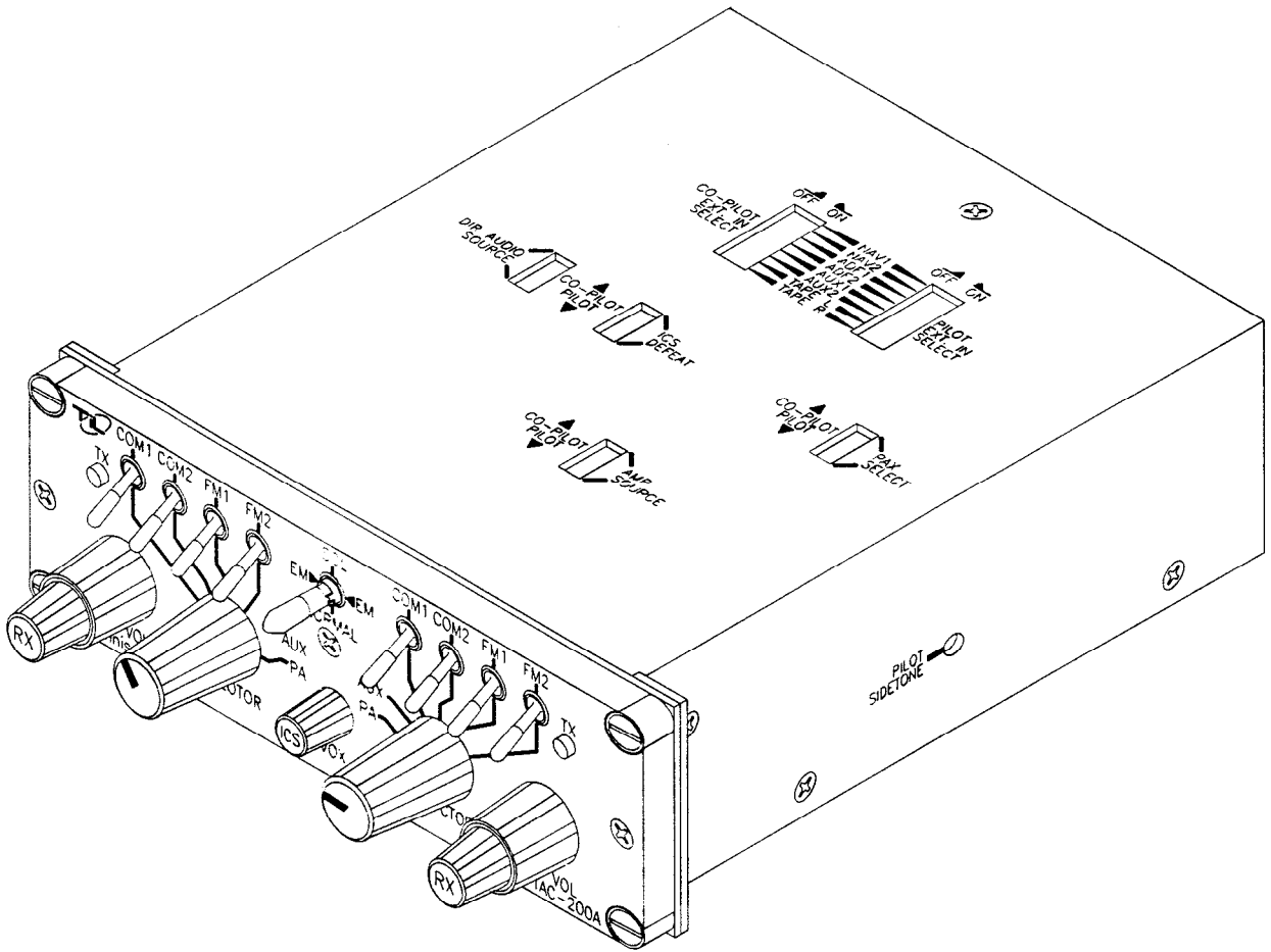
FIGURE I-1 TAC-200A DUAL AUDIO CONTROLLER - GENERAL VIEW
