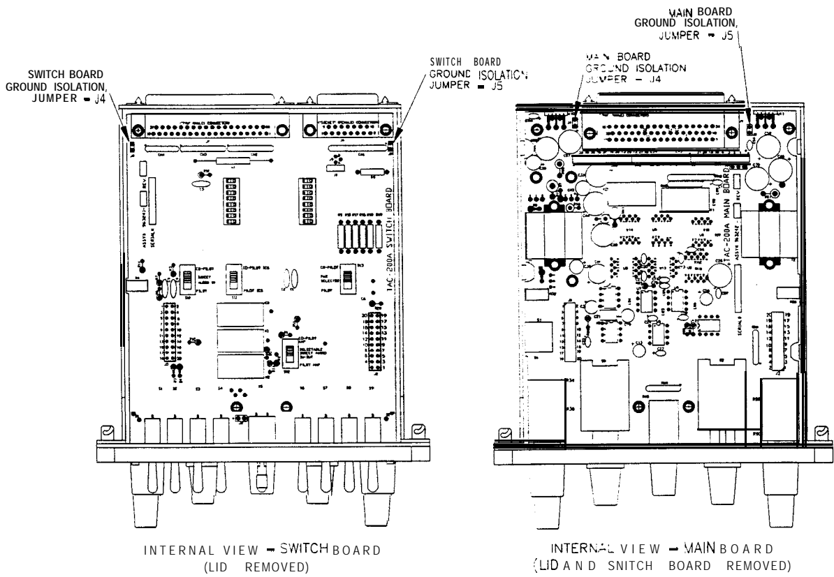
FIGURE 2-6 GROUND ISOLATION JUMPER LOCATIONS
