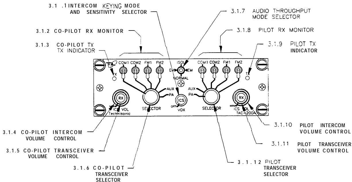
FIGURE 3-1 TAC-200A FRONT PANEL OPERATOR'S SWITCHES AND CONTROLS
