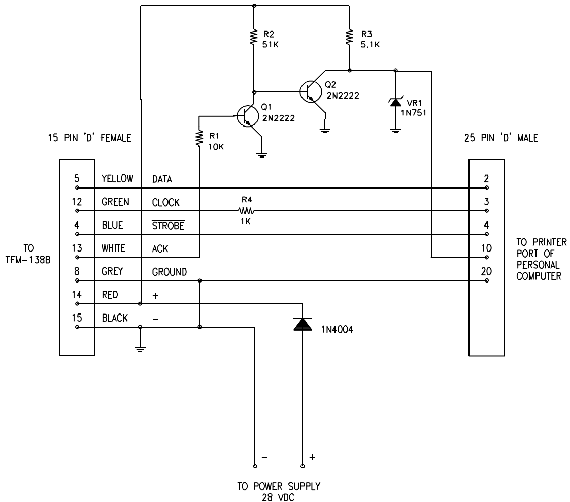
TFM-403 Upload/Download Programming Cable For DOS Program P/N 943165-4 - Wiring Diagram
