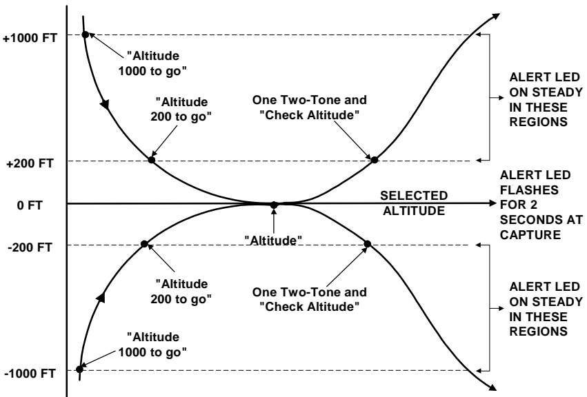
Fig. 4-2. Altitude Selector / Alerter Annunciation Flight Profile
