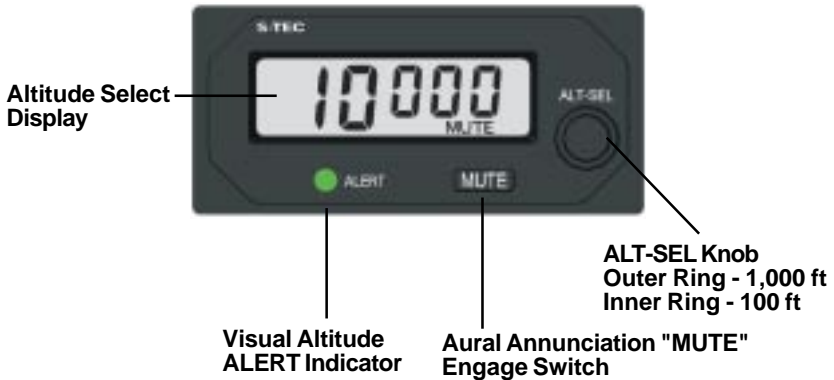
Fig. 3-1. Altitude Selector / Alerter Quick Reference
