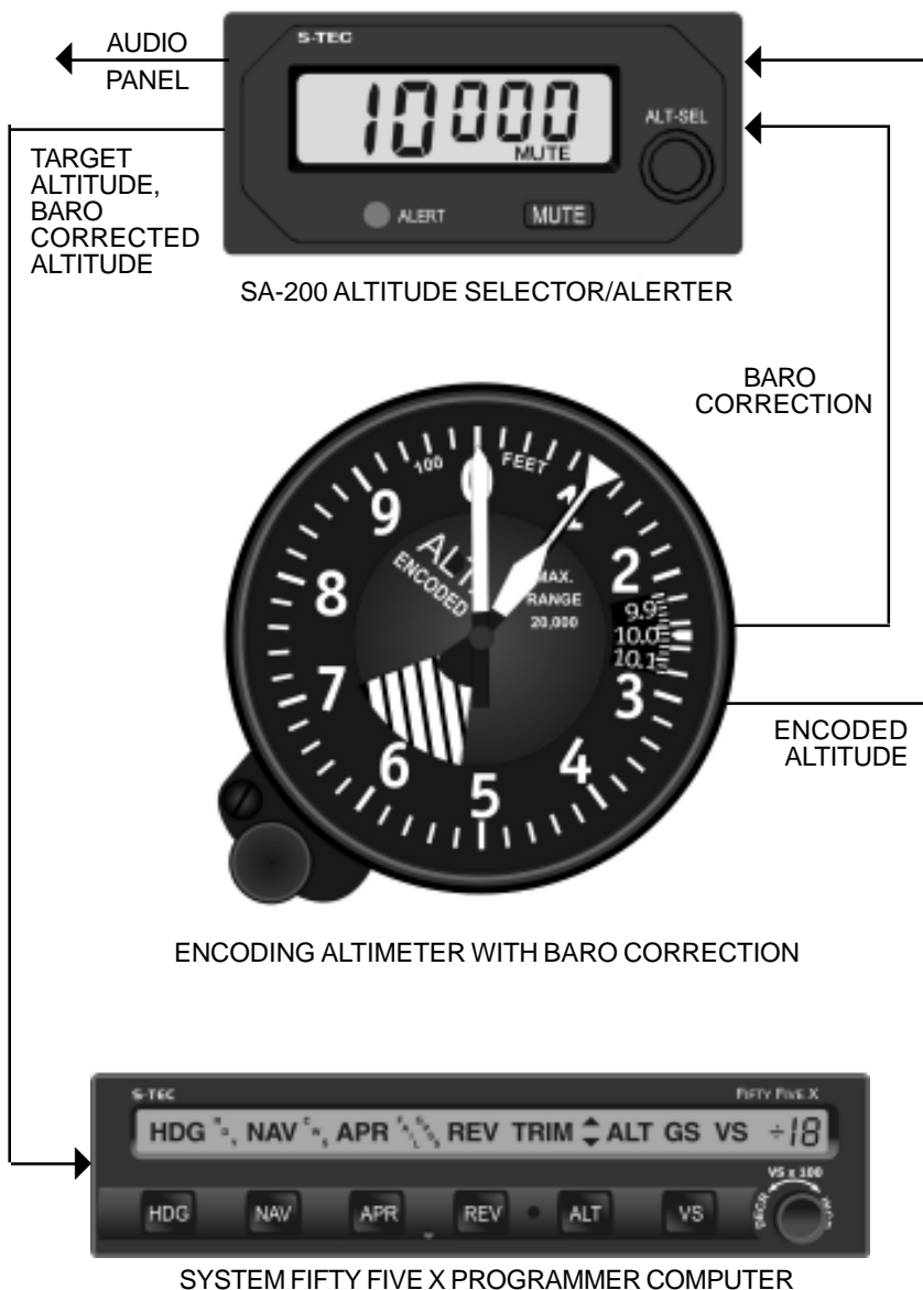
Fig. 2-1. SA-200 Altitude Selector/Alerter Block Diagram
